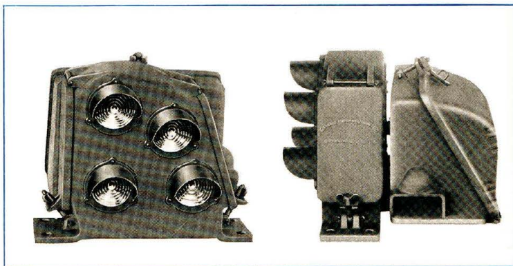
Figure 22 Type C Position-Light Dwarf Signal Unit
