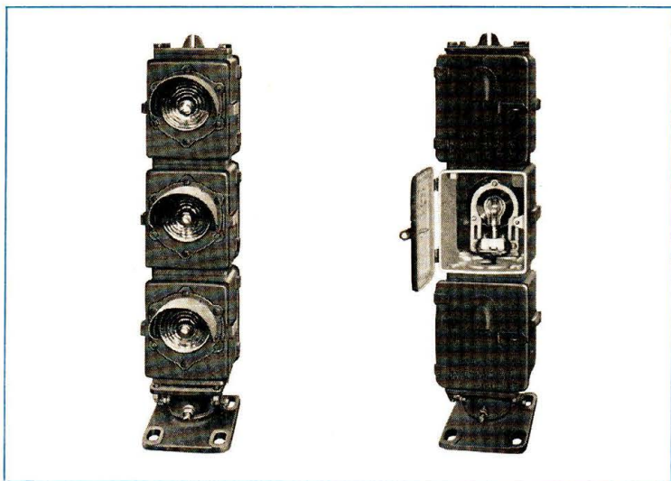
Figure 11 Type F Three-Indication Color-Light Dwarf Signal
