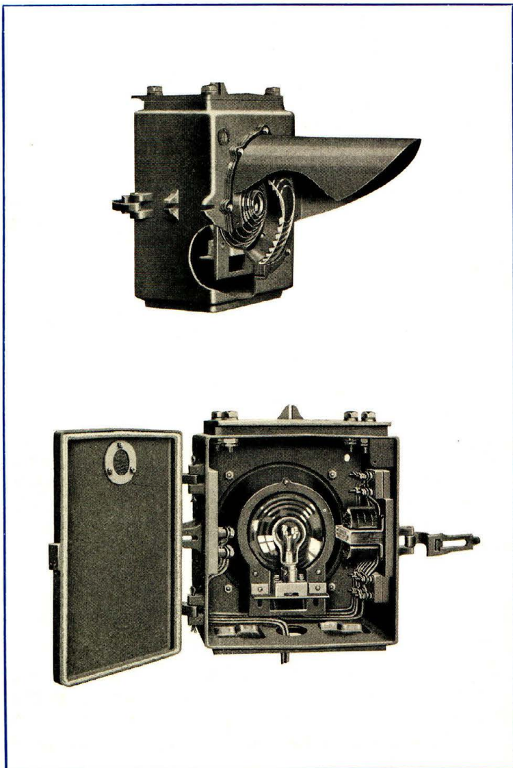
Figure 3 Type D Lamp Case with Doublet-Lens Light Unit
