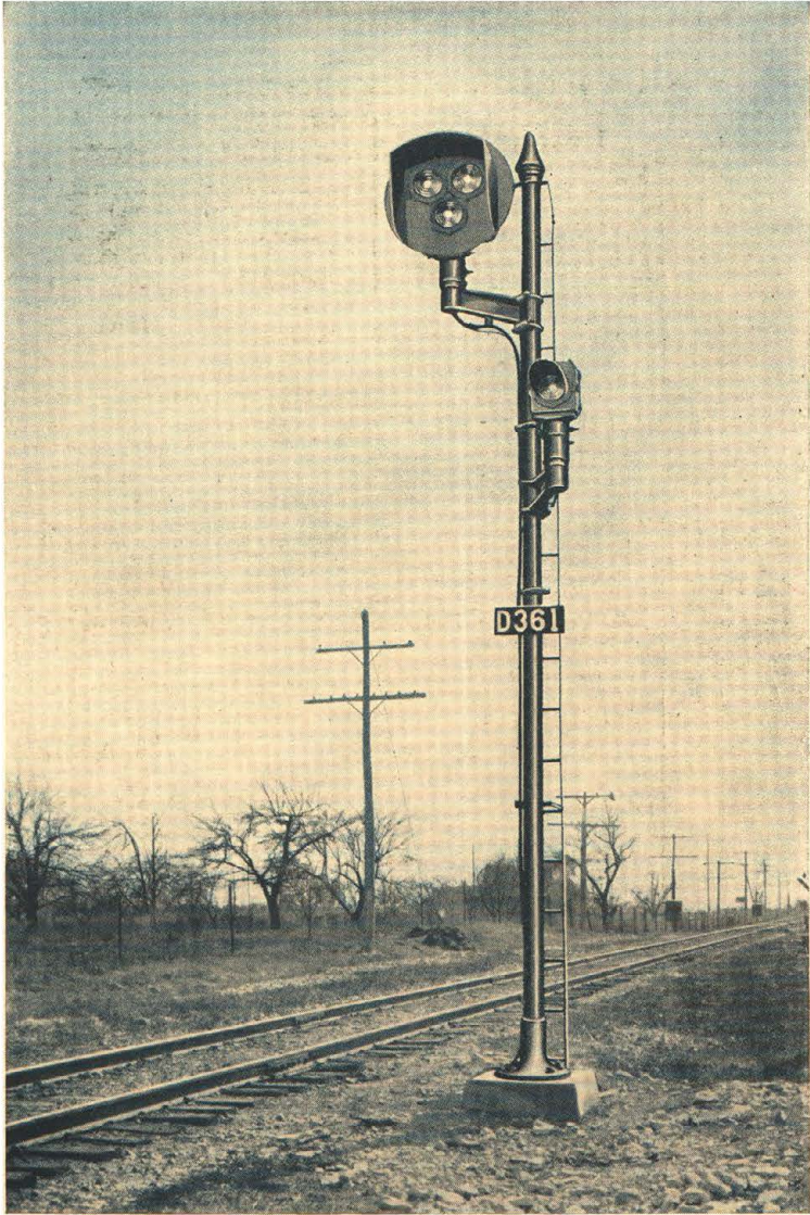
Figure 9 Type G Color-Light Signal Michigan Central Railroad
