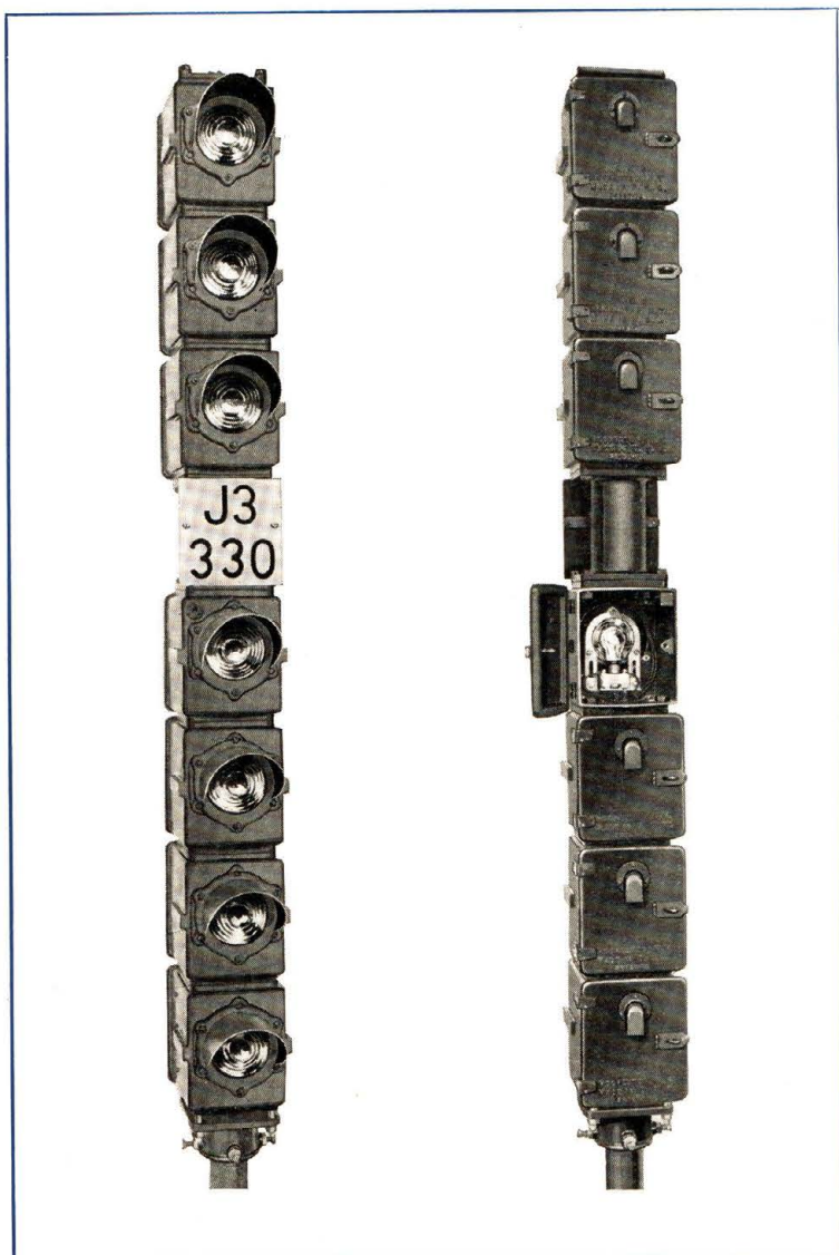
Figure 12 Type F Color-Light Interlocking Signal
