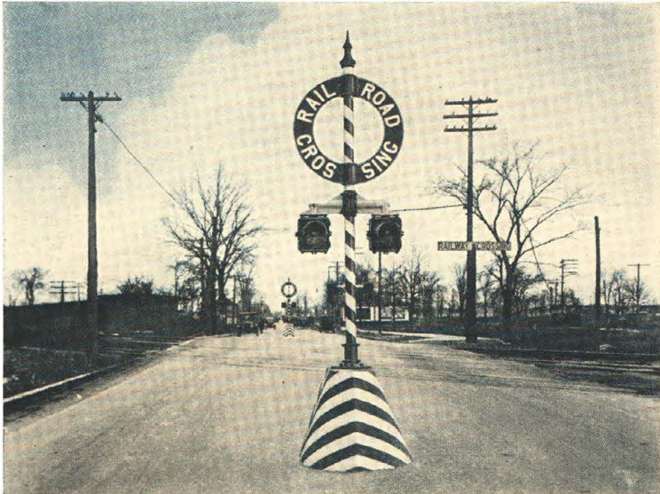
Figure 17 Type K Color-Light Highway-Crossing Signals Grand Trunk Railway System
