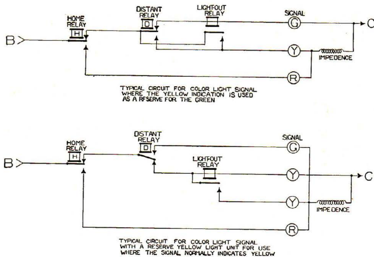
Figure 8 Circuits for Reserve Indications Type E Color-Light Signal
