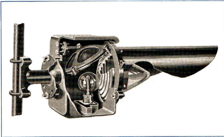
Figure 21 Type B Position-Light Signal Lamp Unit
