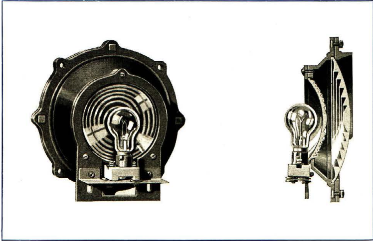
Figure 2 Doublet-Lens Unit
