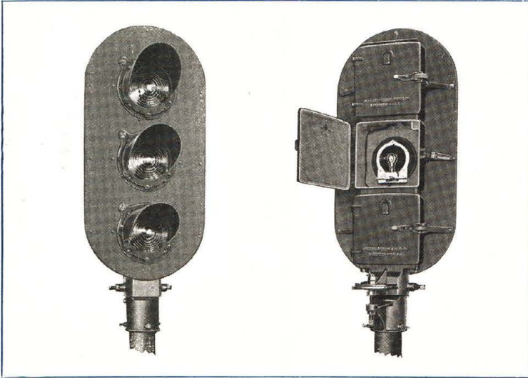
Figure 5 Type D Three-Indication Color-Light Signal Unit
