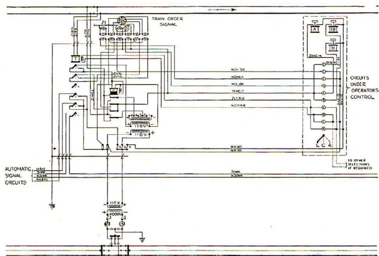
Figure 15 Circuits for the Control of a Combination Train-Order and Automatic Signal
