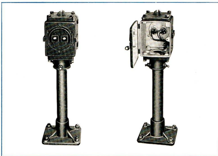
Figure 16 Switch Indicator, Light Type, Two-Indication
