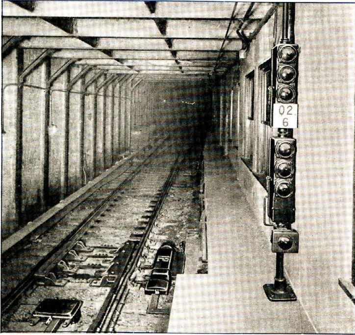
Figure 13 Type A Color-Light Signal Brooklyn Manhattan Transit Co
