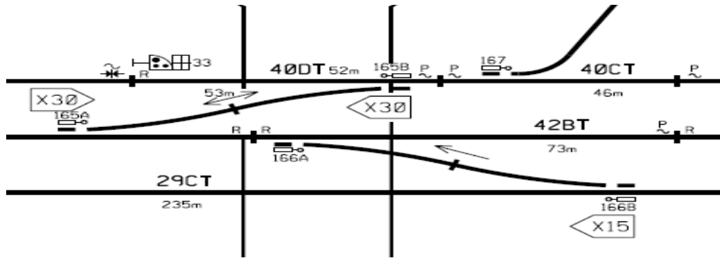
Figure 1 Clearance Point for 33 signal
