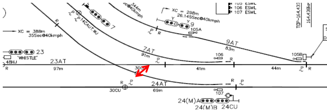
Figure 3 The Signal Arrangement Plan is deceptive as there is not sufficient clearance at this insulated rail joint between 7AT track section and 24AT track section
