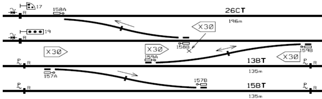
Figure 2 No Clearance Point between 157A points and 159A points
