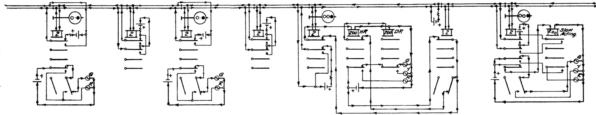
TRAFFIC ONE DIRECTION-TWO INDICATION SIGNAL BACK OF THREE INDICATION SIGNALS.
