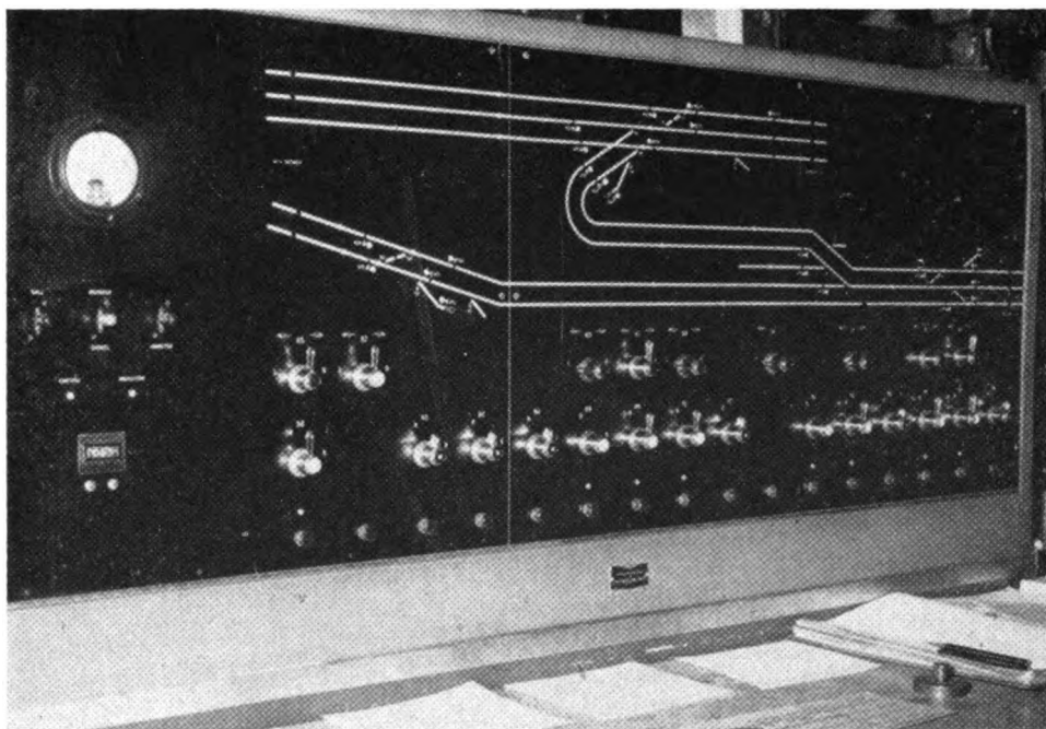
Control machine for Bay City Junction Interlocking
