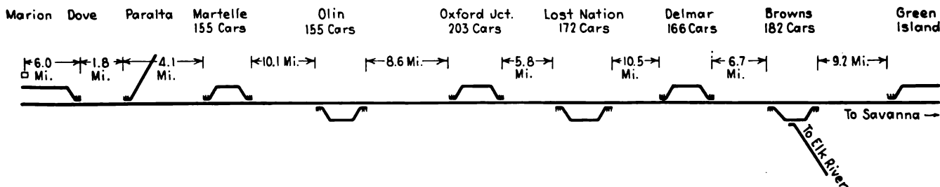
Layout of new single track main line and sidings on the 67 miles of road
