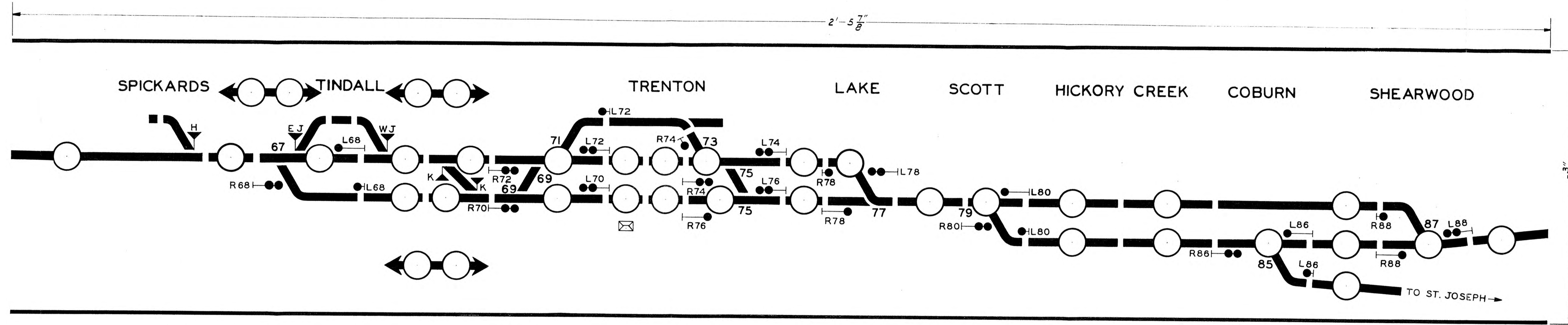
TRACK MODEL PLATE FOR C.R.I. & P.R.R. ALLERTON-TRENTON INSTALLATION GEN. DWG. 179592-C9388-SH. 1.
