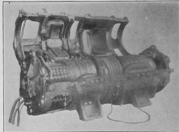
Westinghouse 3000-Volt, 85-Volt Motor Generator Set
