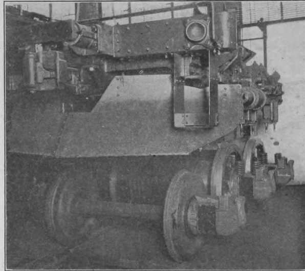
Leading Truck Partly Assembled, Showing Wedges in Place on Journal of Guiding Axle
