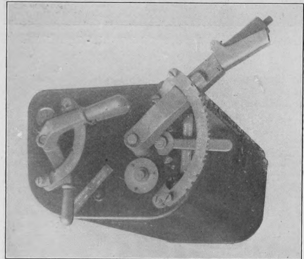
Top View of Westinghouse Master Controller
