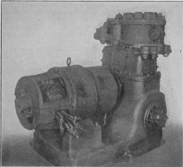
Air Compressor Driven Through Gears and Cranks by 30 HP. Motor
