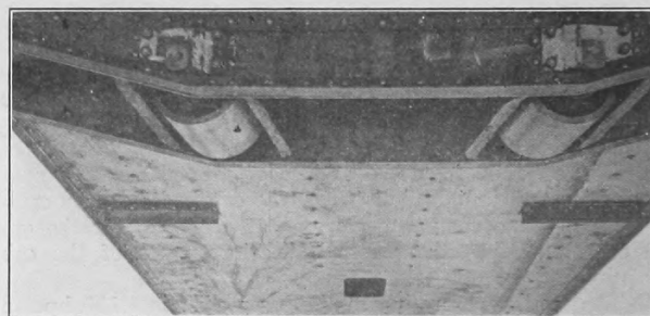
Platform and Rollers Which Constitute Upper Half of Centering Device
